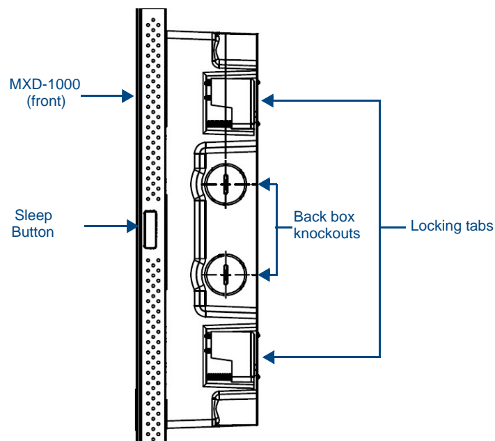
FIG. 14 Side view of MXD-1000 (Portrait)
