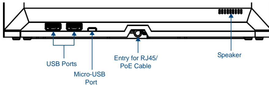
FIG. 3 MXT-1000 USB port location
