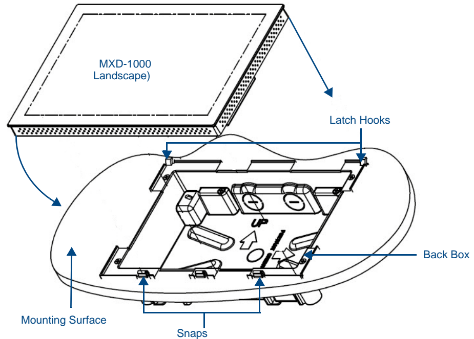
FIG. 19 Installing the MXD-1000
