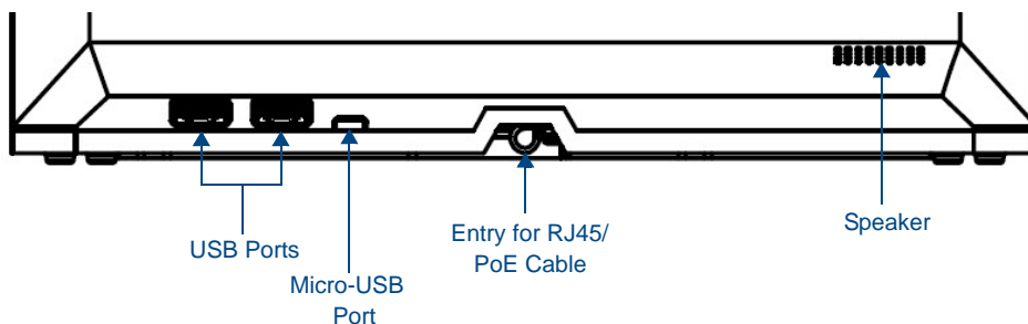
FIG. 9 Connectors on the rear of the MXT-1000
