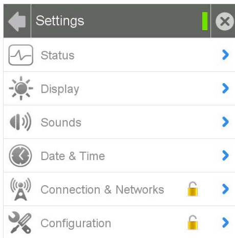
FIG. 23 Settings page
