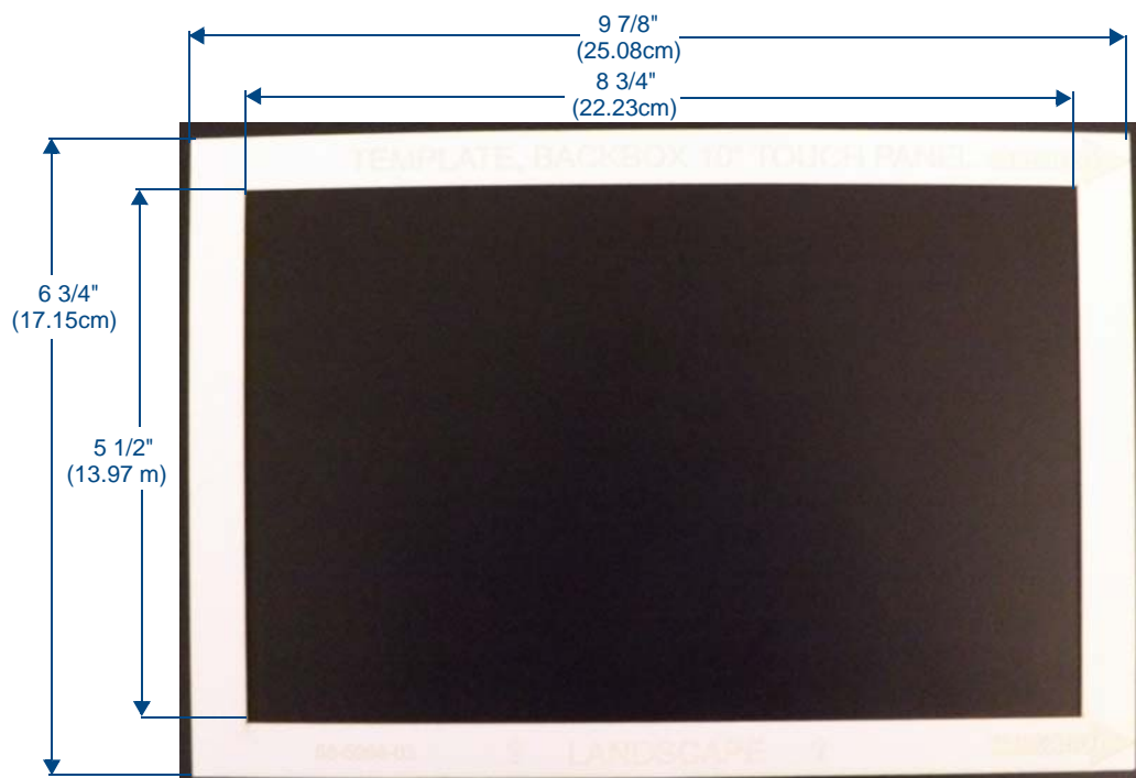
FIG. 15 MXD-1000 Installation Template
